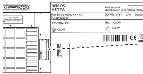
W Placement product label, wall-mounted product
